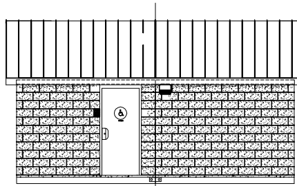
① FRONT ELEVATION 24 GA DUAL PITCH MODEL C
