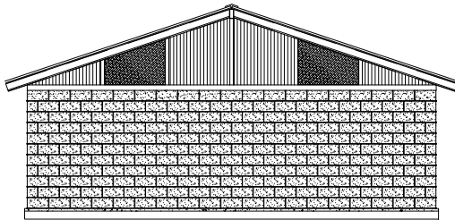
② SIDE ELEVATION 24 GA DUAL PITCH MODEL D
