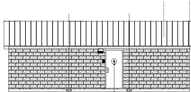
① FRONT ELEVATION 24 GA DUAL PITCH MODEL D
